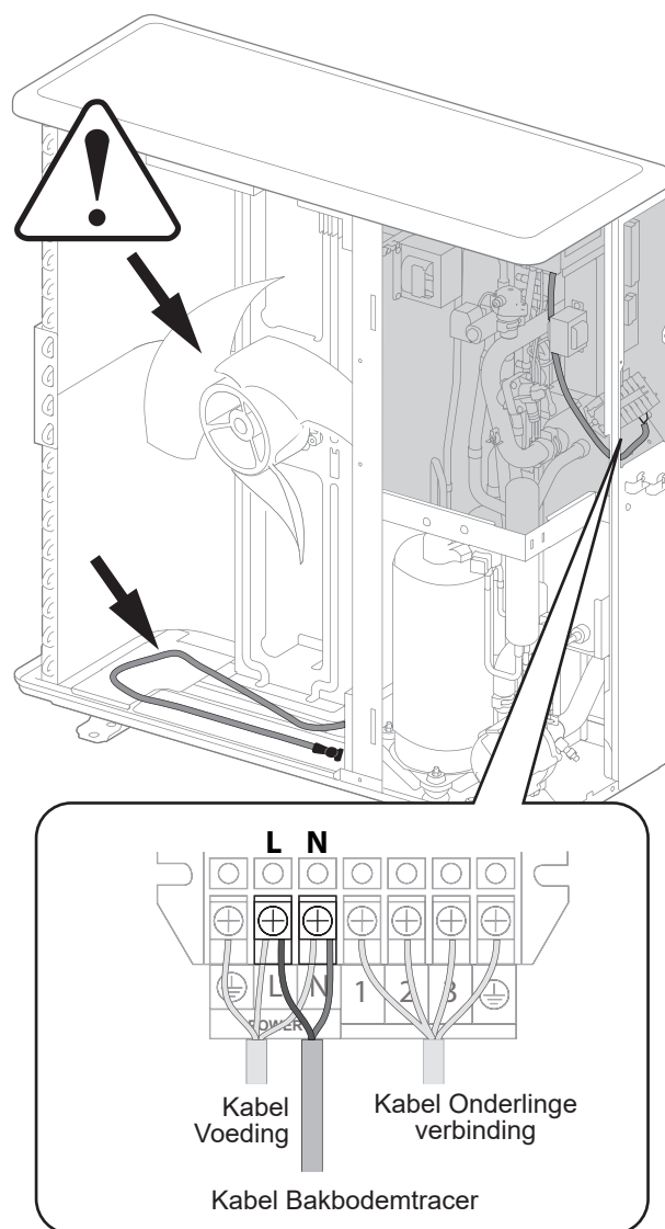
fig. 42 - Montage bakbodemtracer
