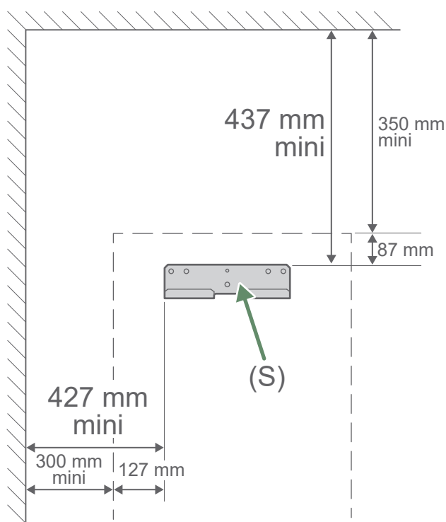
fig. 20 - Wandmontage
